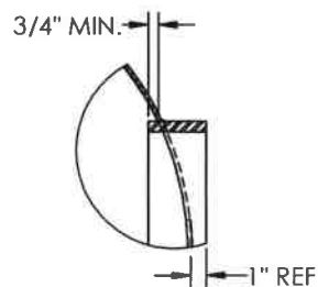
MANWAY DETAIL
